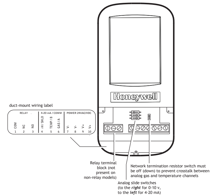
Figure 3: wiring the duct-mounted monitor
