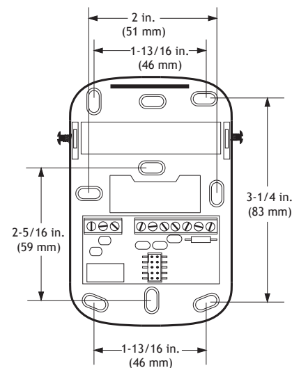
Figure 1: Backplate mounting hole distances (9 holes)
