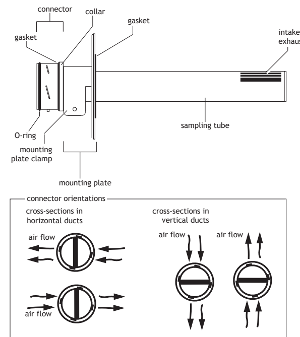
Figure 4: sampling tube and mounting plate
